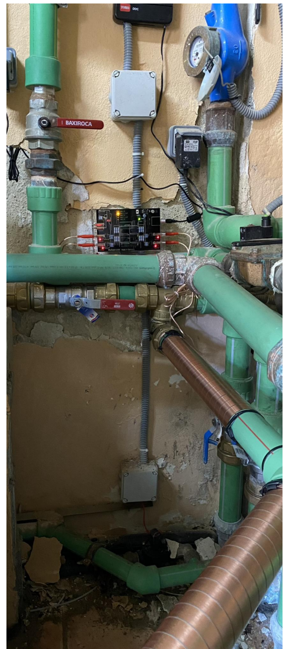
Vulcan S50 in the cold water pipe with Ø 63 mm
